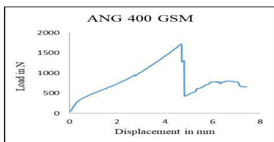
Fig 1.7 Graphical Result for ANG laminate
